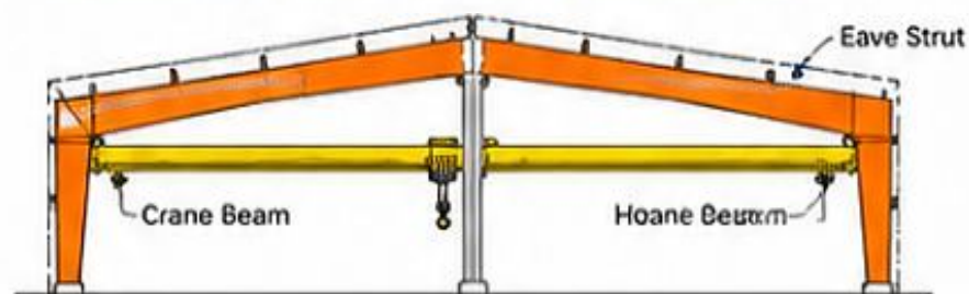
Top Running Crane in a Multi-span Building
